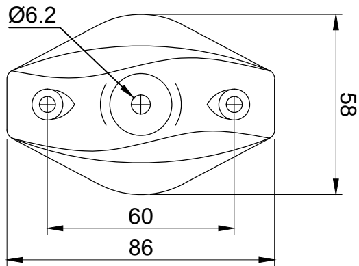
Movable Mounting Flange
